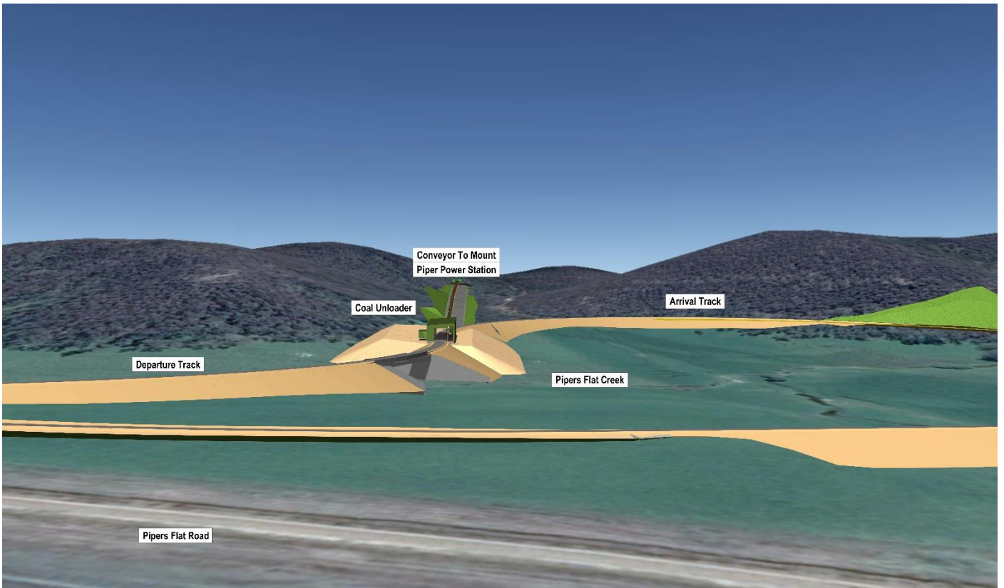
Figure 3. View looking north towards unloader and conveyor
