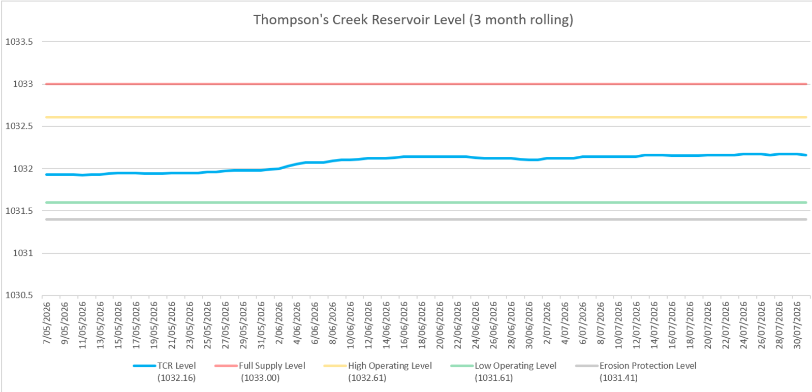
Figure 7: TCR Water Level
