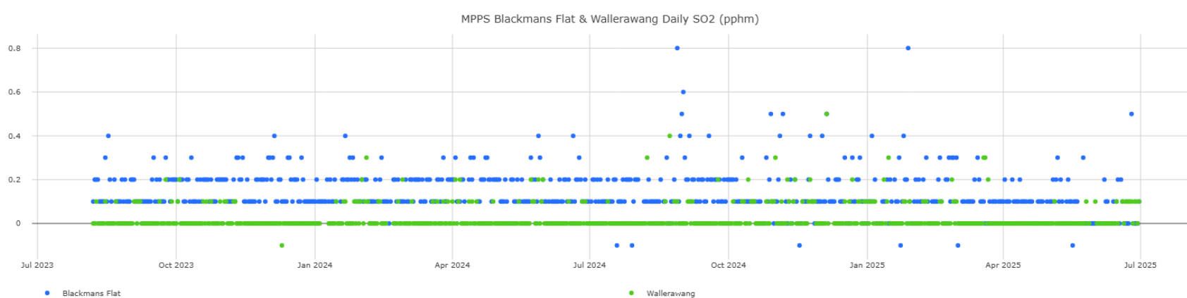
Figure 6: MPPS SO2 pphm Daily Average
