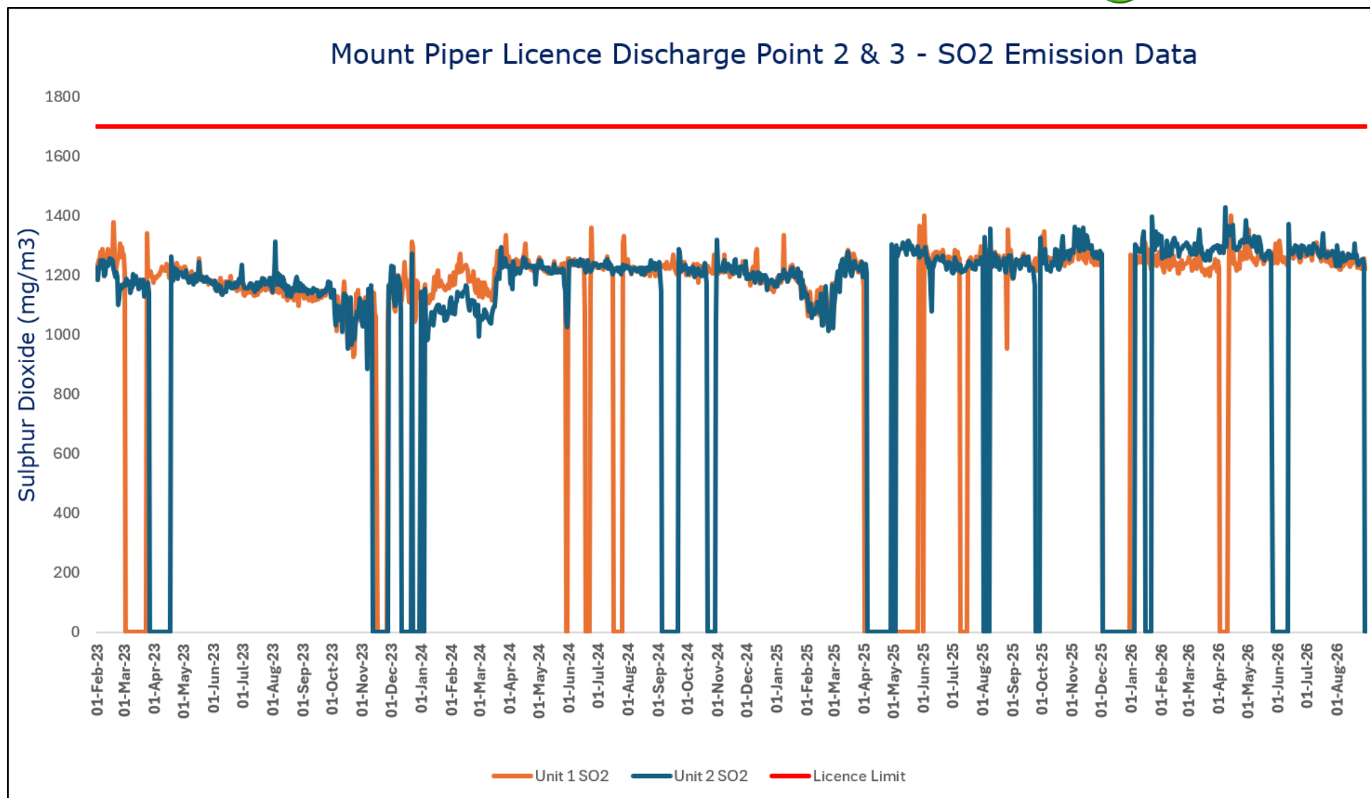
Figure 2: Sulphur Dioxide (SO 2 ) Emission Data
