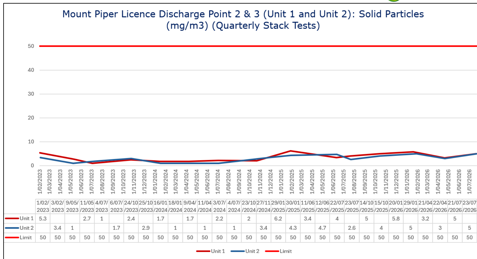
Figure 3: Solid particles Emission Data
